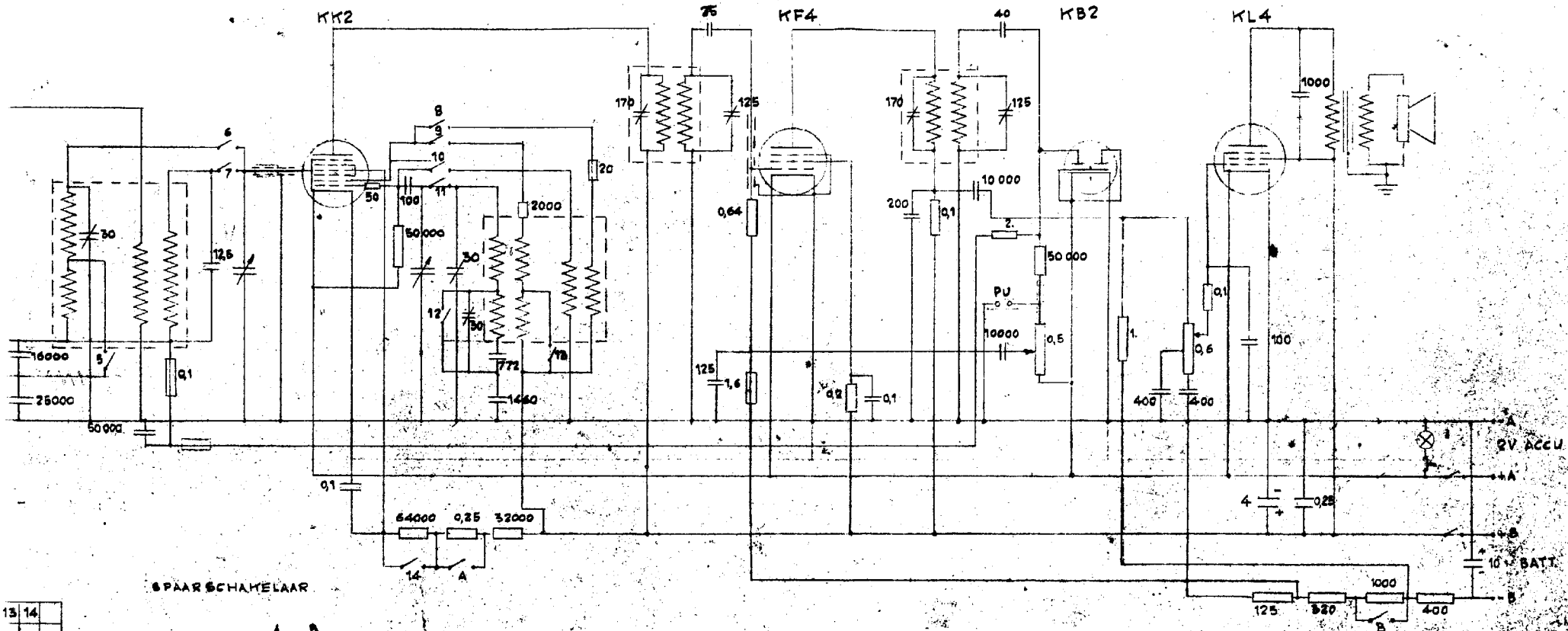
SCHEMA APP. TYPE 108 WALDORP RADIO
